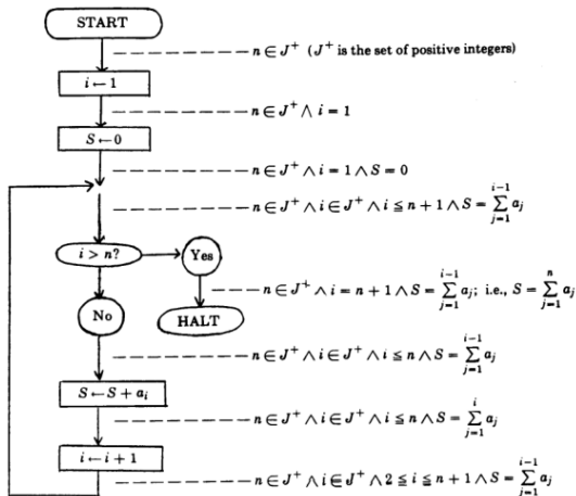
FIGURE 1. Flowchart of program to compute S = \sum_{j=1}^{n-1} a_j ( n \geq 0 )
